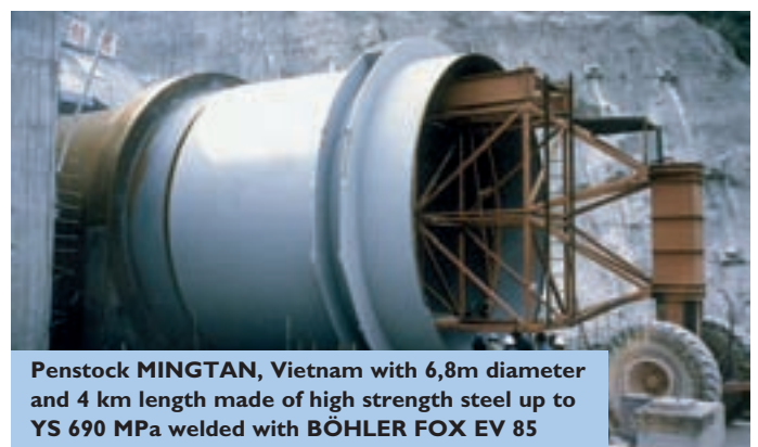
Prefabrication of the Penstock Kaprun, Austria Steel grade S 690 Q, ASTM A514 Gr.F, SAW BÖHLER 3NiCrMo2,5UP+BB24
